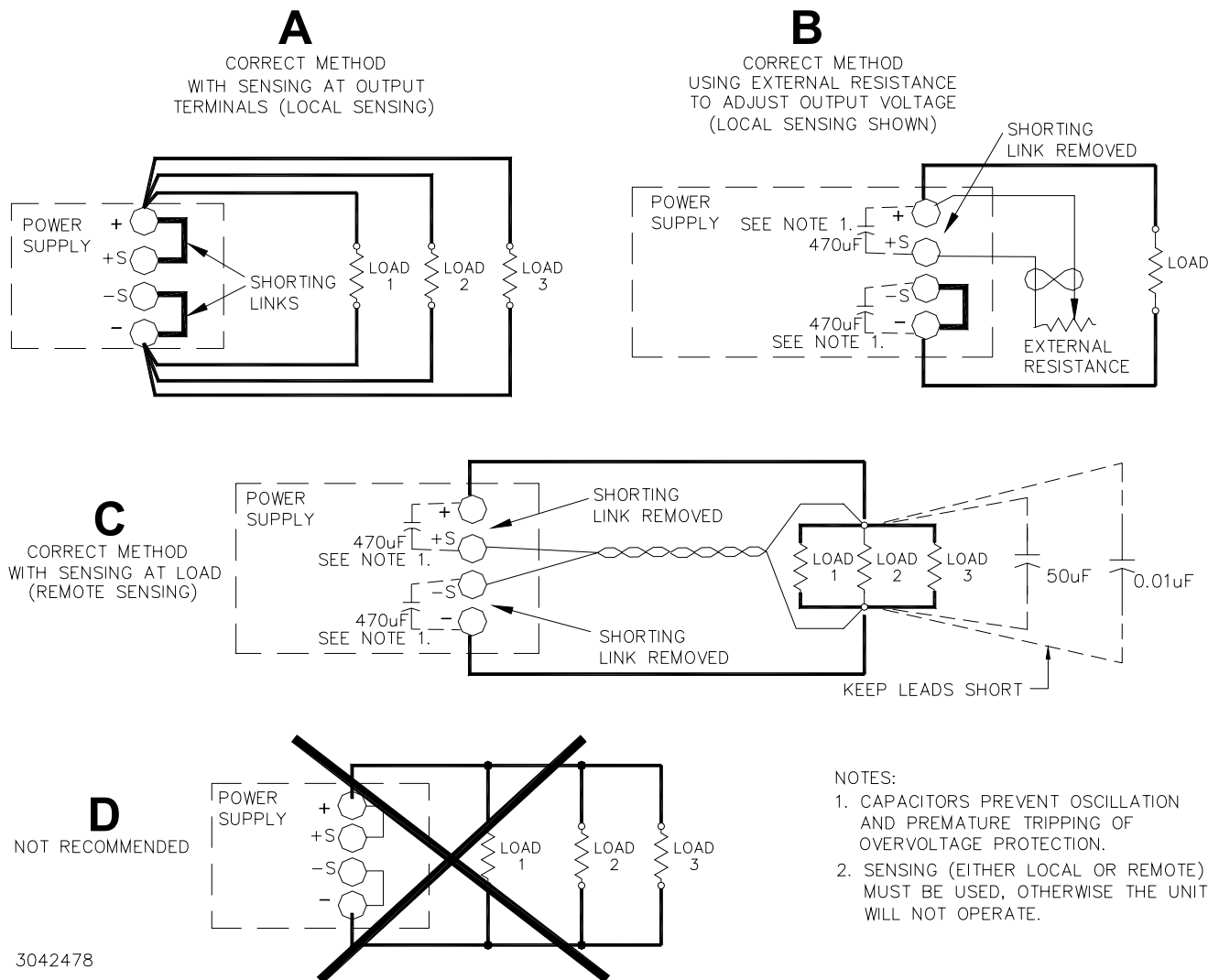
FIGURE 3. LOAD CONNECTIONS
