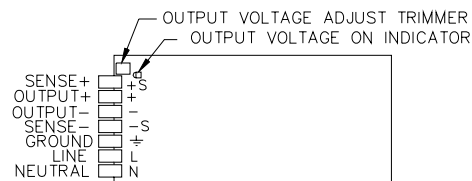
FIGURE 2. COMPONENT LOCATIONS
